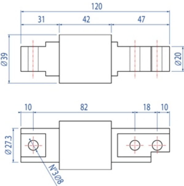
Dimensions (mm)
