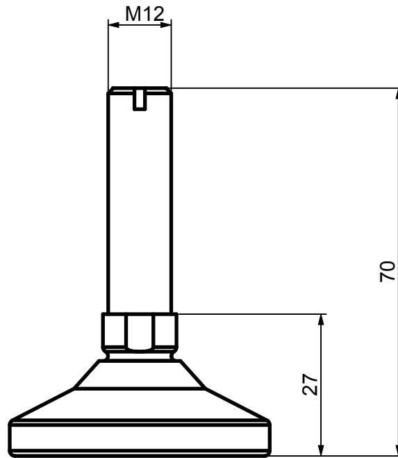
SBF1 Dimensions in mm.
